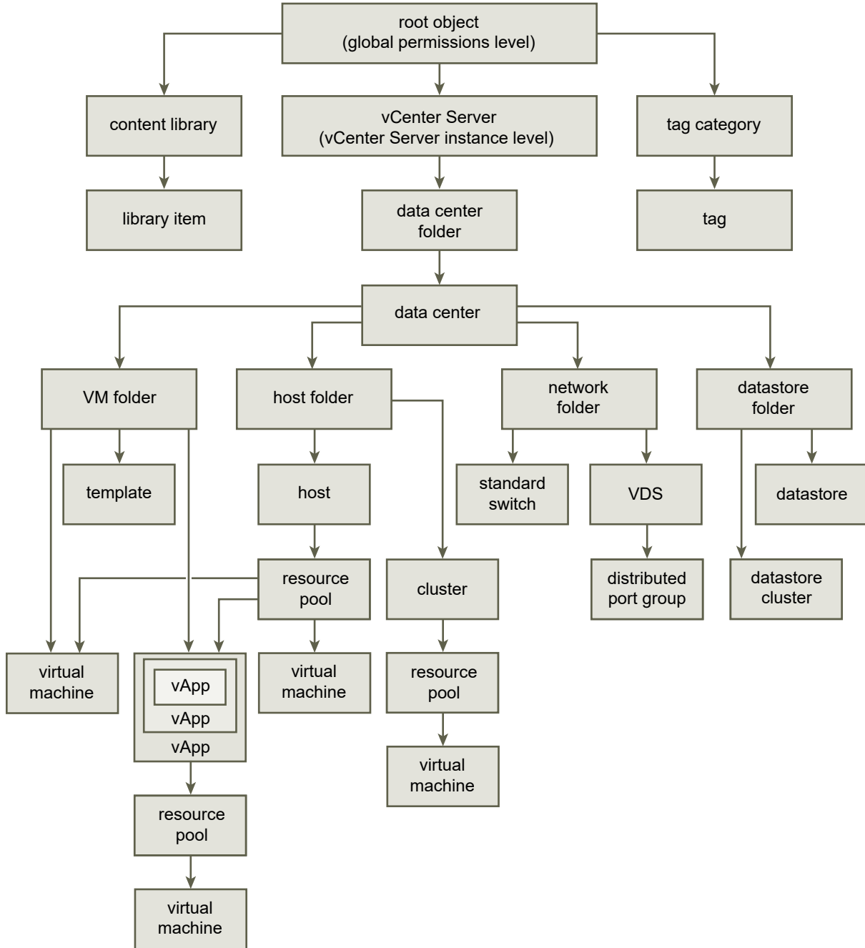
Figure 5-1. vSphere Inventory Hierarchy
